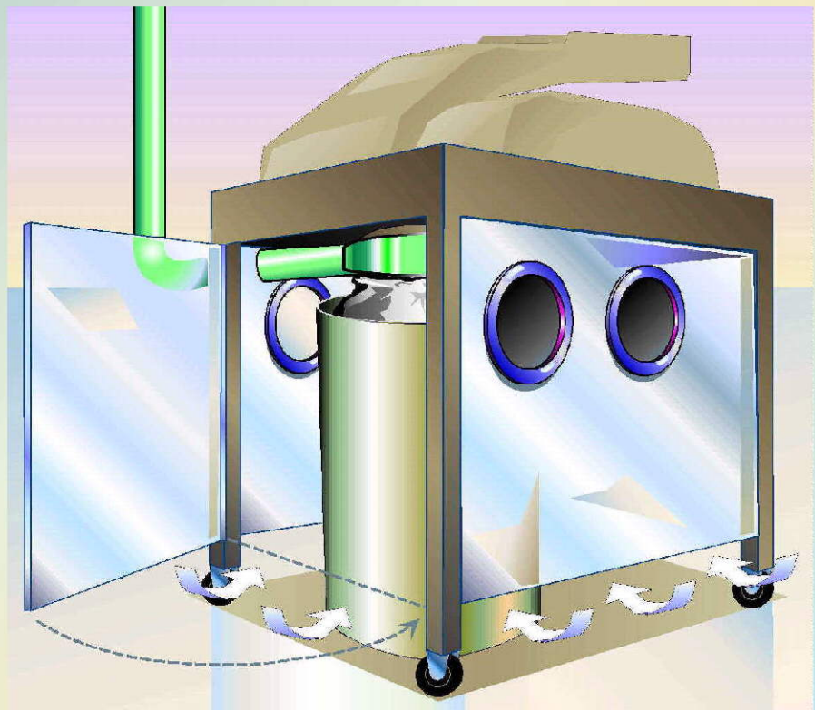
Chloroform and Wax Mixing Cabinet and Drum Enclosure for Tablet Coating
